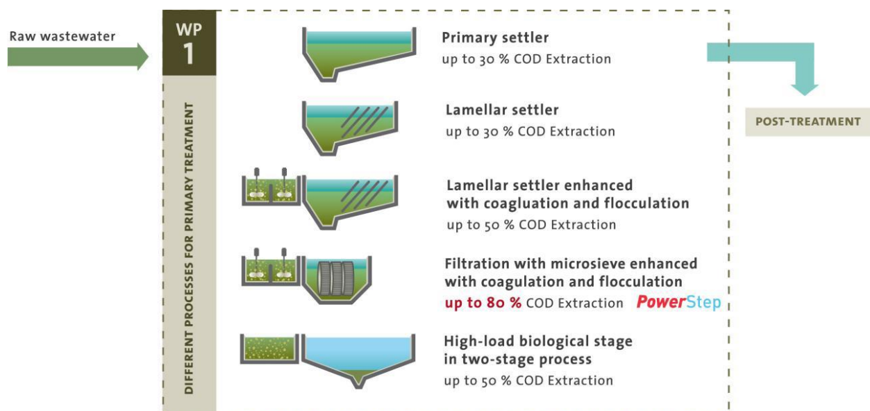
Figure 5: Wastewater treatment process scheme with different primary treatment options
