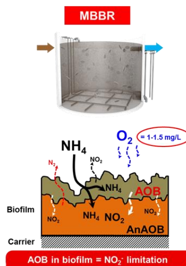
Figure 1: The concept of one-stage deammonification in the MBBR configuration
