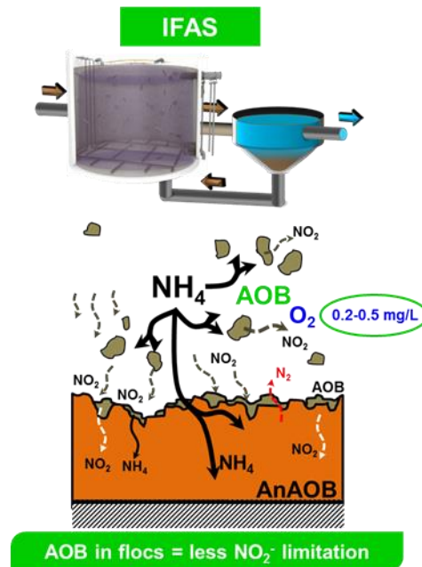
Figure 3: The concept of one-stage deammonification in IFAS MBBR configuration
