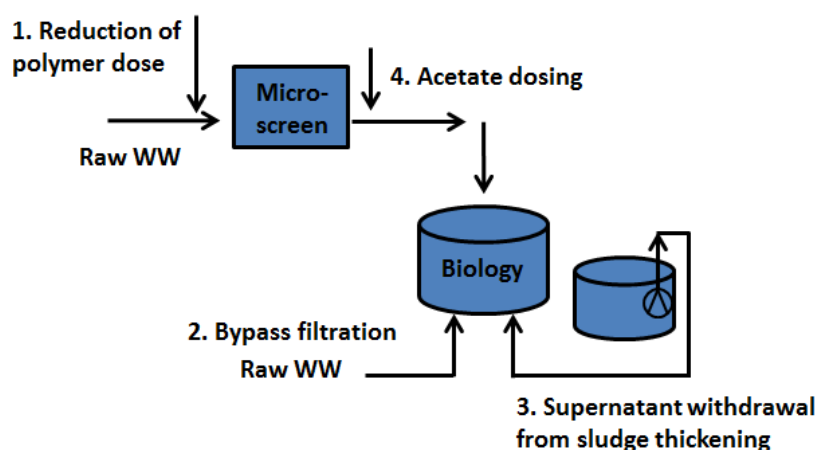
Figure 6: Schematic description of special mechanisms for advanced nitrogen control applied after microscreen
