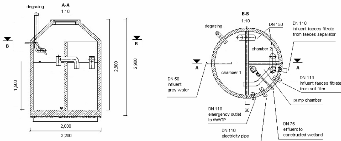
Fig. 2.4.14: Septic tank
