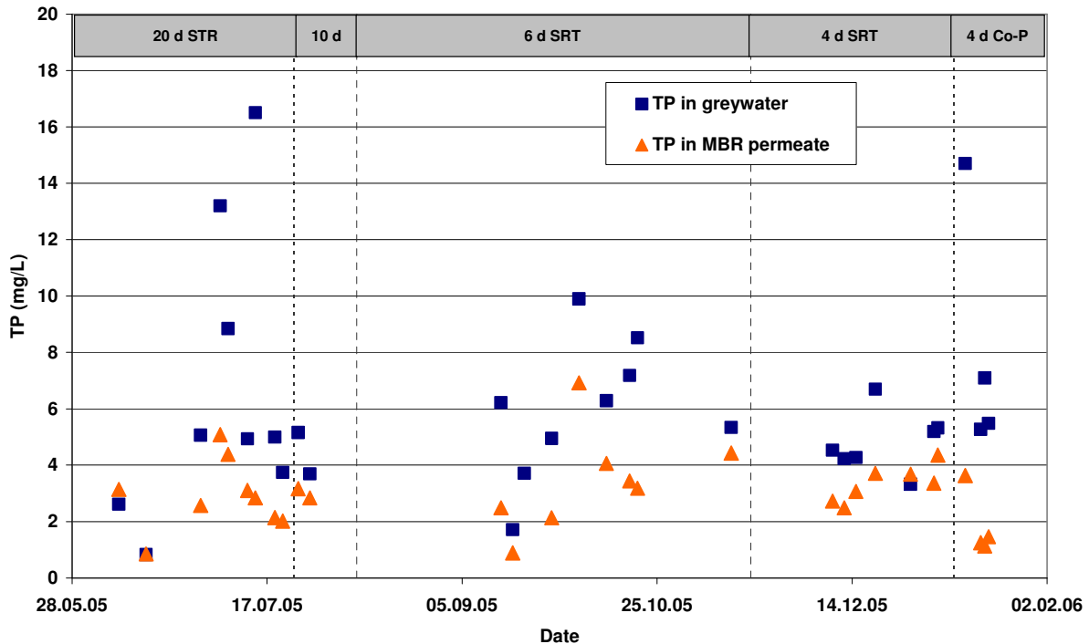
Fig 3.5.7.5: TP concentrations in greywater and in MBR permeate
